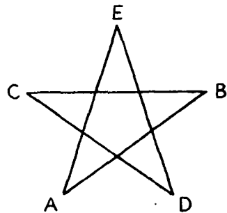
FIGS. 7 and 8. Kepler (Fig. 7) shaded each face in a different way to show which triangles belong to the same pentagonal face.
