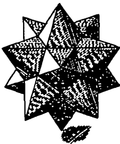
FIGS. 7 and 8. Kepler (Fig. 7) shaded each face in a different way to show which triangles belong to the same pentagonal face.
